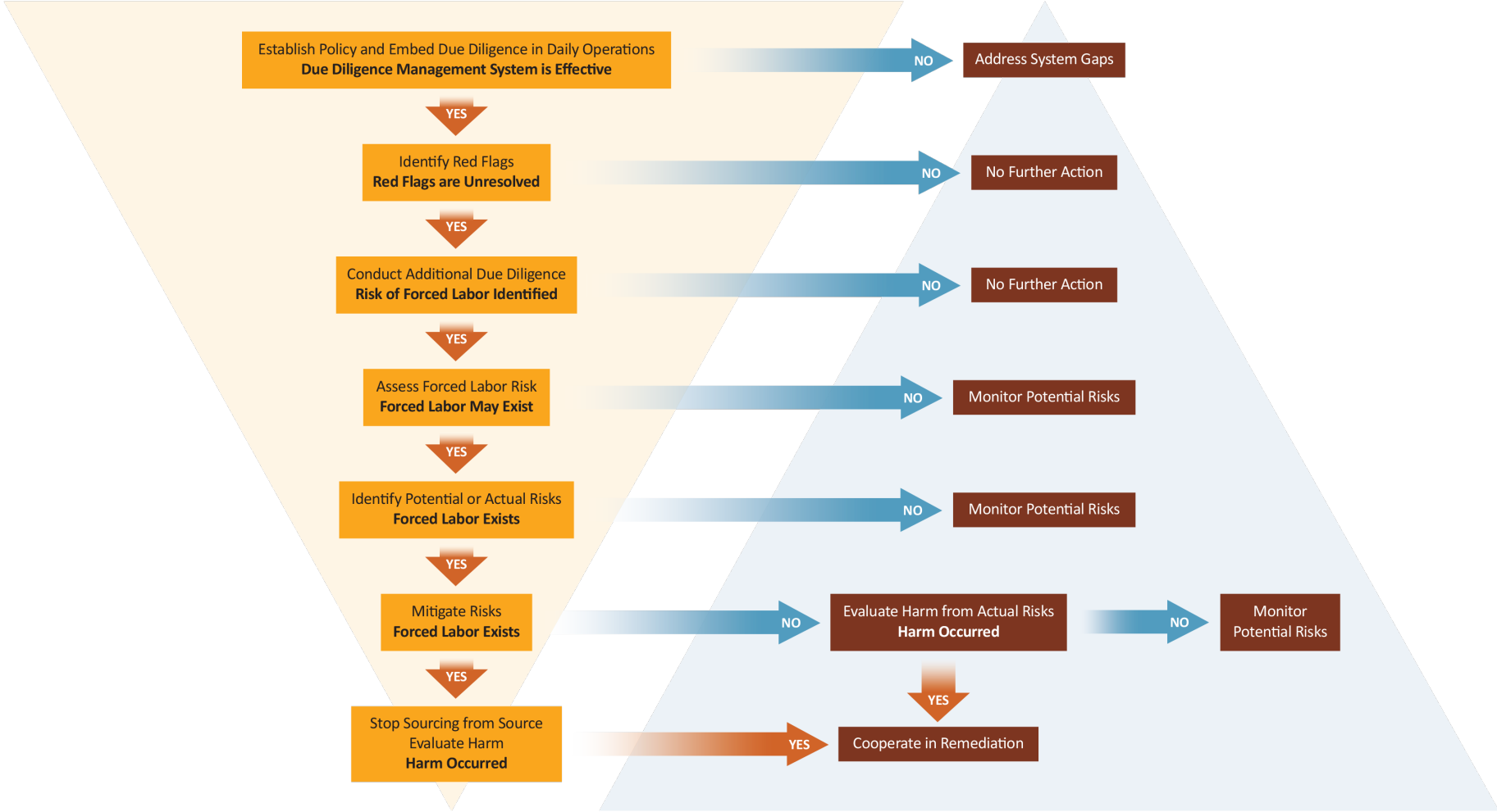
Figure 1: High-Level Due Diligence Process Decision Tree
